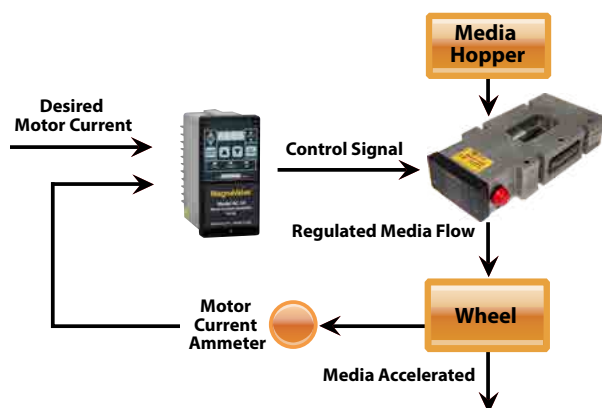
Closed Loop System with AC-24 Controller
