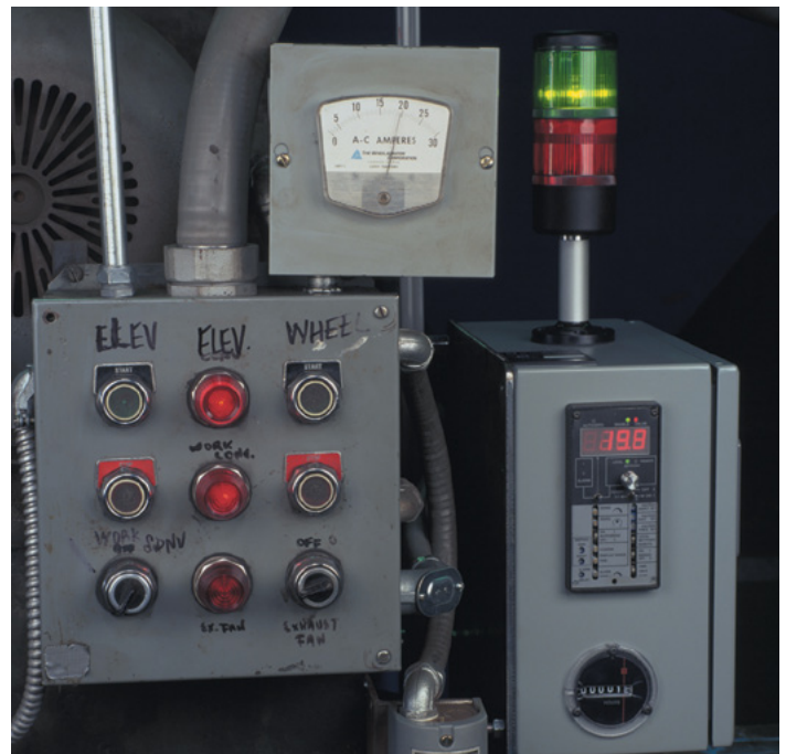
Figure 19. Final setting at 20 amps
