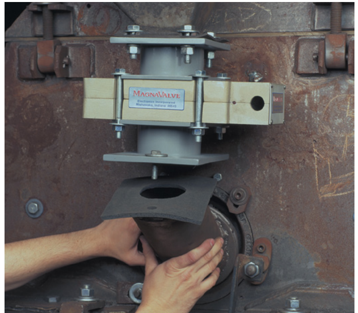
Figure 11. Re-install feedsput to wheel
