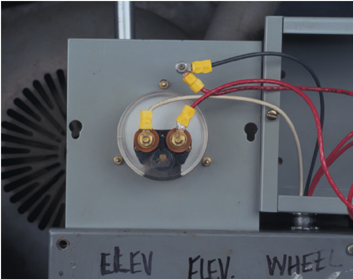
Figure 15. Splice for AC Controller shunt
