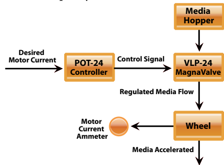
Figure 2. Open-Loop: Magnetic Valve
