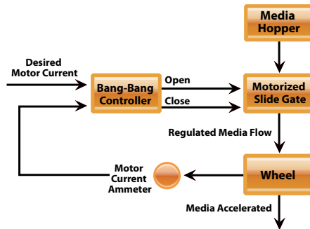
Figure 3. Closed-Loop: Motorized Slide Gate
