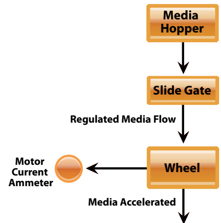
Figure 1. Open-Loop: Manual Slide Gate
