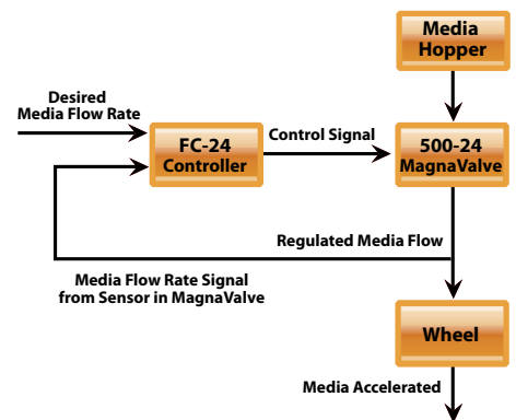
Figure 5. Closed-Loop Magnetic Valve (flow rate)
