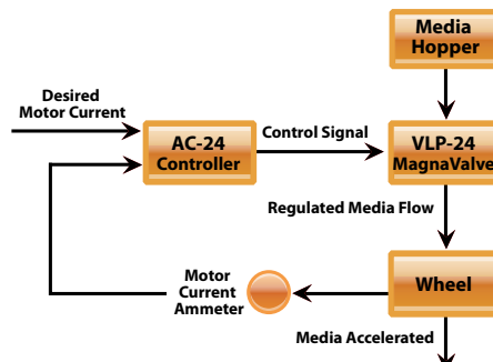
Figure 4. Closed-Loop Magnetic Valve (motor current)
