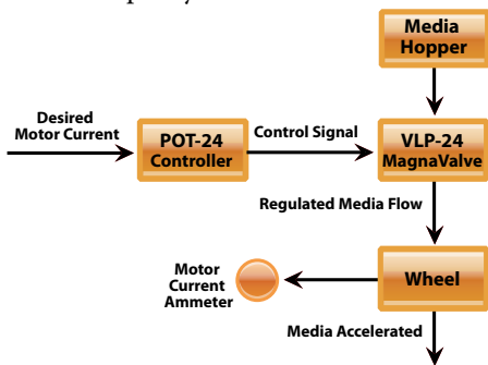
Figure 2. Open-Loop: Magnetic Valve
