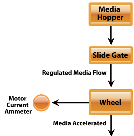
Figure 1. Open-Loop: Manual Slide Gate
